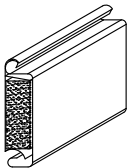
Type 'Ti' Insulated Slat EPS Foam / PVC Back 2 5/8" x 13/16" (Model MI)
