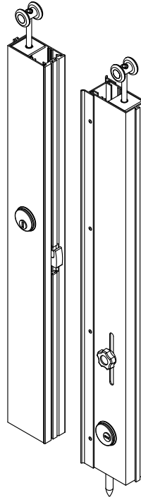
Lead & Reciver Posts Hook Lock & Bottom Lock (Bi-Parting Closures)
