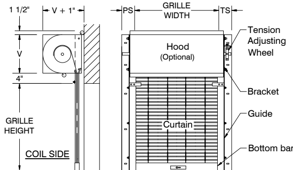
Type 'Z' Guide
