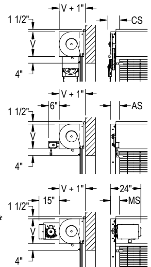
Tube Mount Guide*
